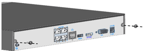
Figure 4-2 Side Panel
